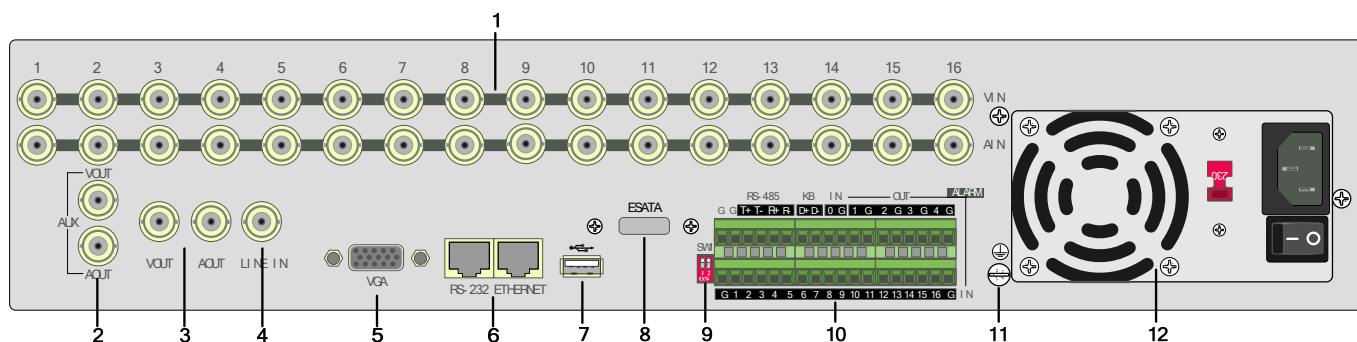
DS-8016HCI-S/DS-8016HFI-S Rear Panel
