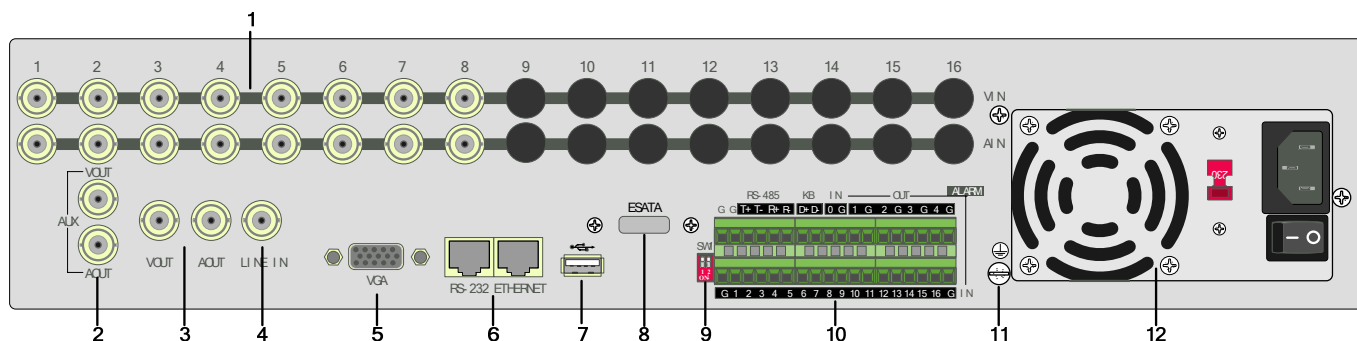
DS-8008HCI-S/DS-8008HFI-S Rear Panel
